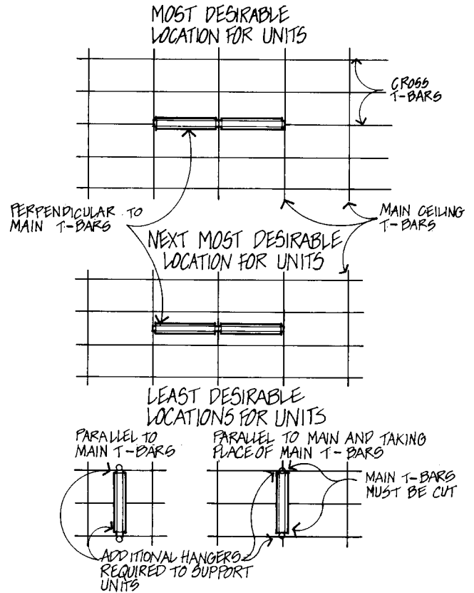
Fig. 15 — Terminal Location
